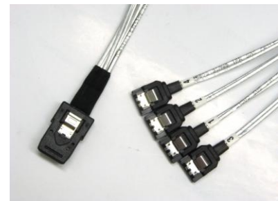
AMPH-874S-XXX: SFF-8087 to 4 SATA2 Cable with XXX as the standard or customized length in cm
